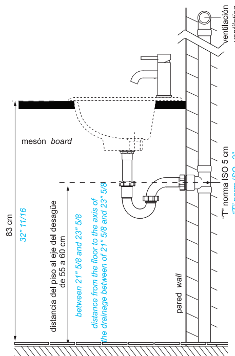
Vista lateral - lateral view
